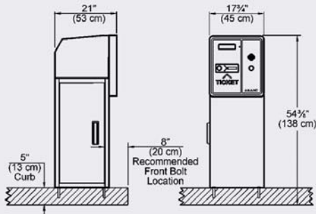
BOLT LAYOUT
